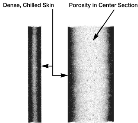
Fig. 7-5 In a thin walled die casting, the fine-grained dense “skin” is a large percentage of the section—with such a section containing virtually no porosity. In a thick section the dense “skin” represents a small percentage of the wall.
