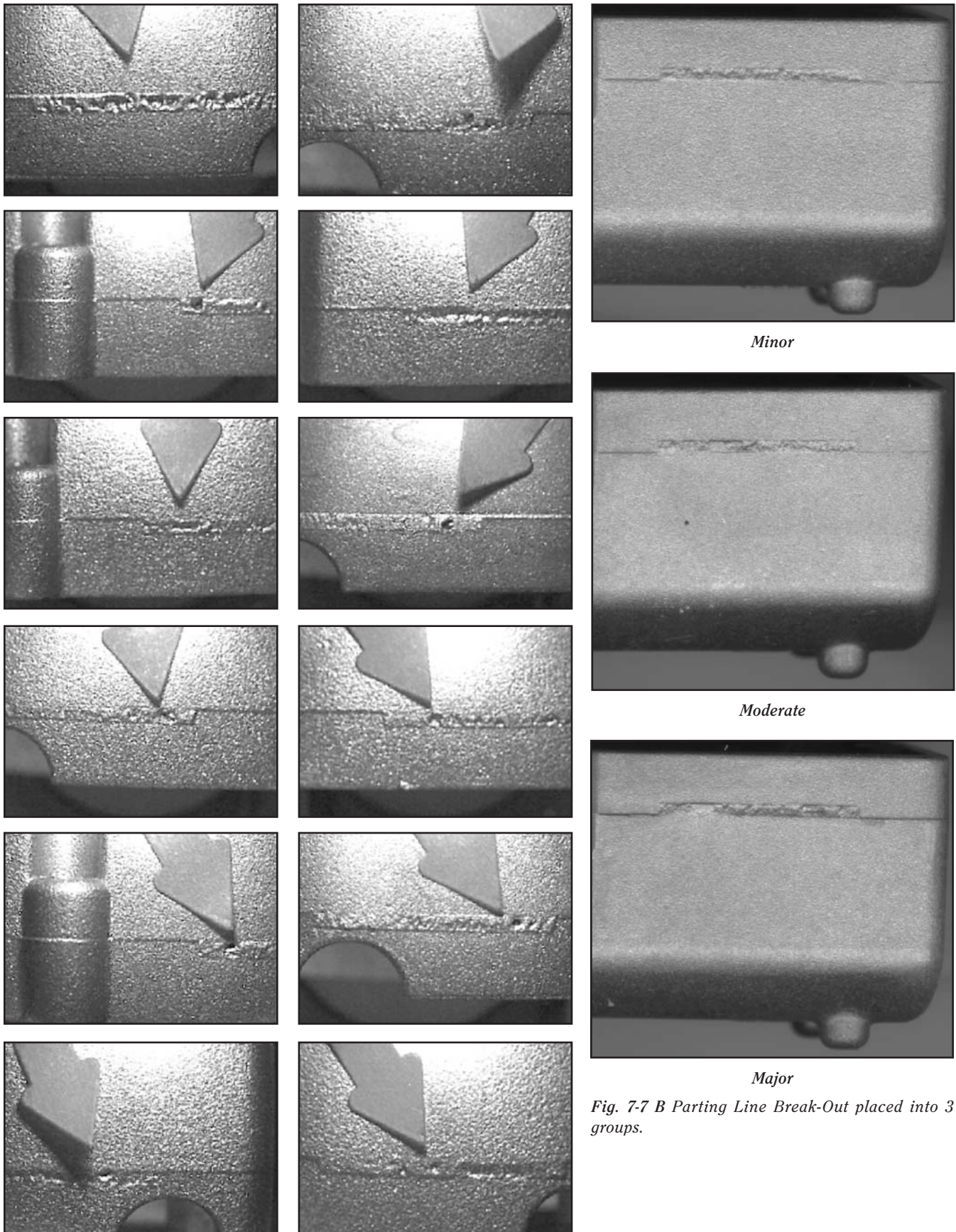
Fig. 7-7 A Parting line porosity at various severity levels.
