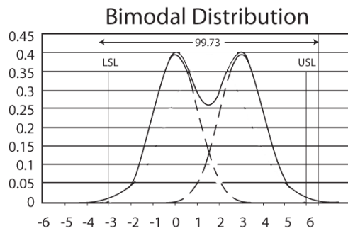
Fig. 7-3 Cp can be applied to a bimodal distribution that allows for migration from one side of the tolerance range to the other. The higher the Cp number the more repeatable the process is.
