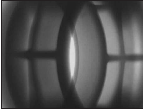
Fig. 7-8 A Example radiograph of a casting with no visible porosity revealed by radiography. This level of soundness is achievable through consultation with your die caster and good part design, process design and process monitoring.
