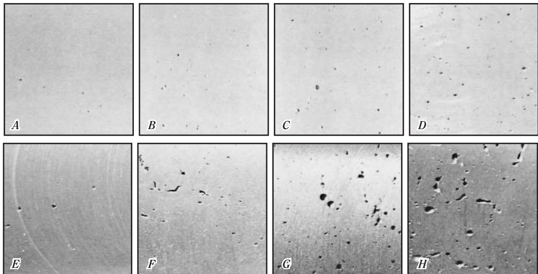
Fig. 7-6 Various degrees of porosity exposed after machining.
