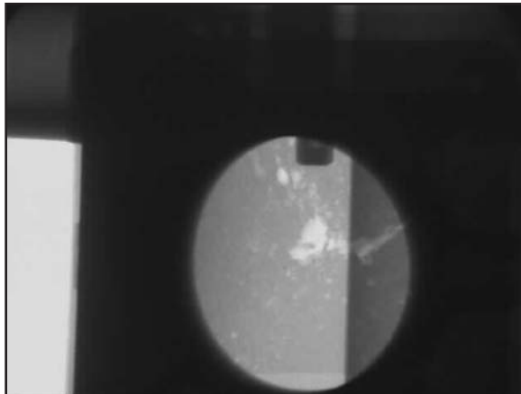
Fig. 7-8 C Example radiograph of shrinkage in a thick cross-section.
