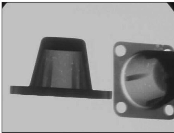
Fig. 7-8 B Example radiograph of porosity that does not impact part form, fit or function. The user should be agreeable to accepting a specified amount of porosity in areas of the casting where it does not impact form, fit, or function.
