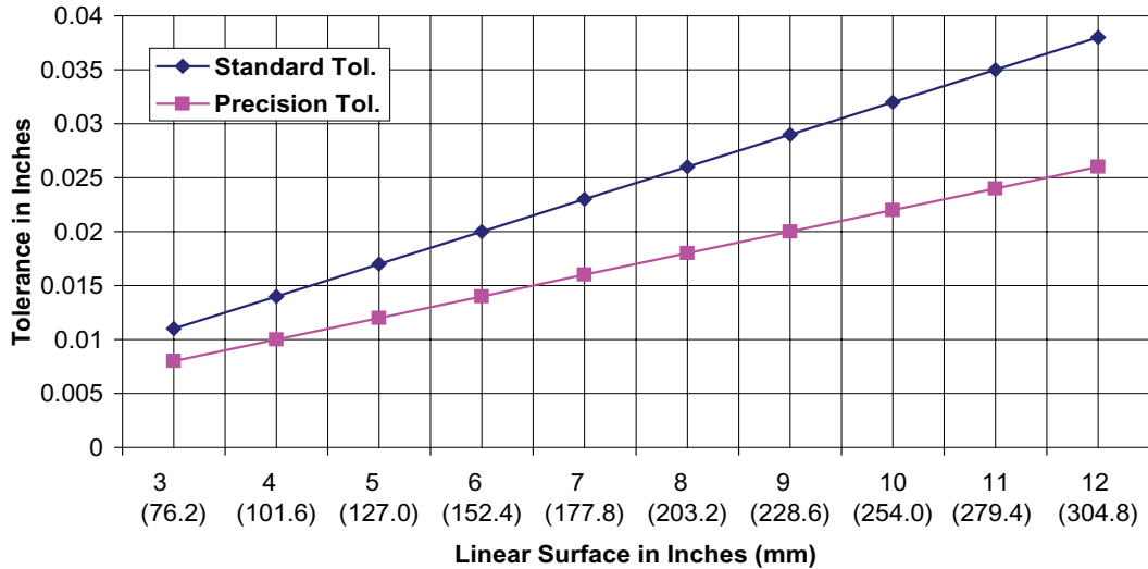
MDC Angularity Tolerance Across Parting Line
