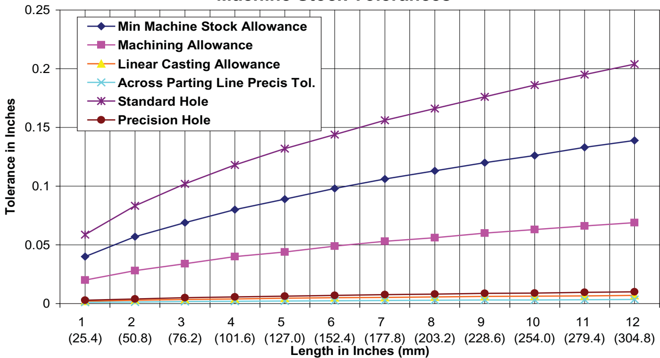
Machine Stock Tolerances
