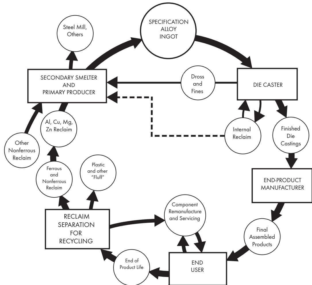
Fig. 1-1 The Die Casting Recycling Circle – The die casting alloy recycling stream, illustrated above, is based on an existing worldwide metal reclamation infrastructure that has been operative for more than 40 years. This basic recycling pattern, with variations based on the amount of reclaimed alloy going to secondary and primary producers, applies to the majority of die castings being currently specified.
